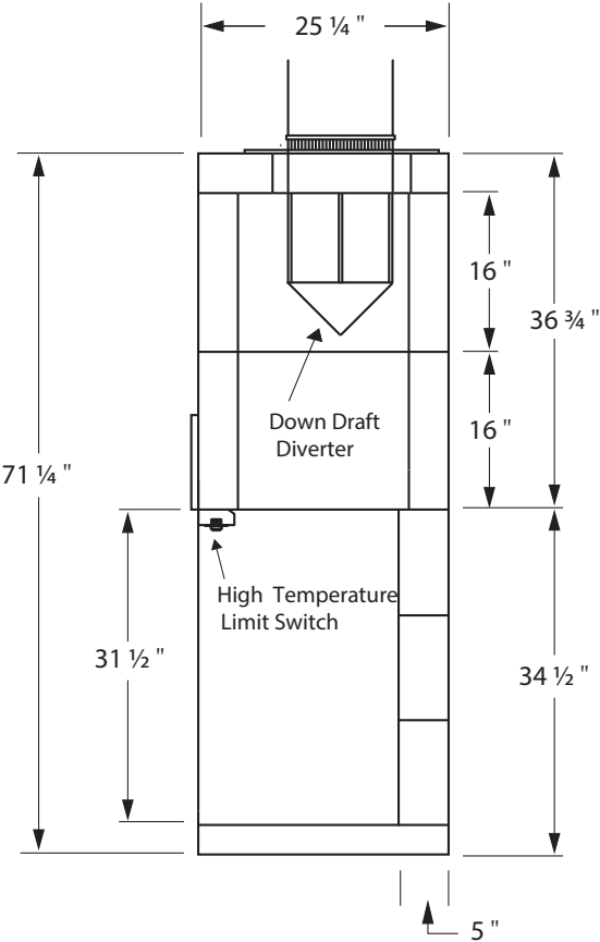
Side View
