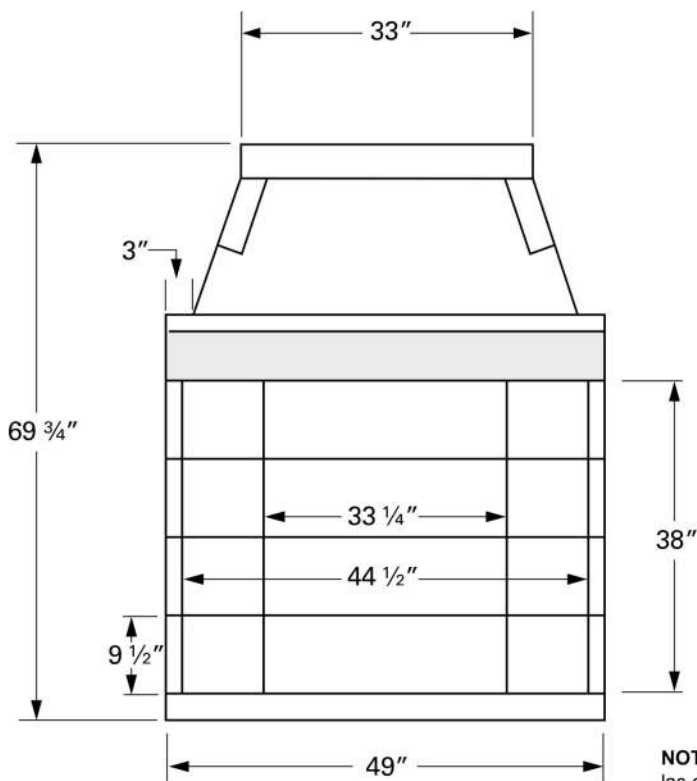
Vista frontal
