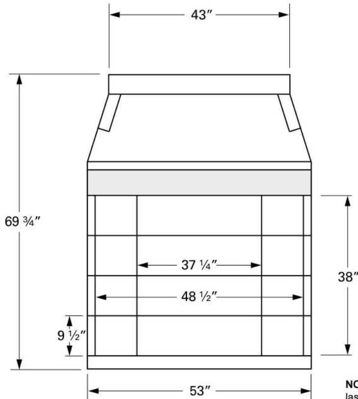
Vista frontal
