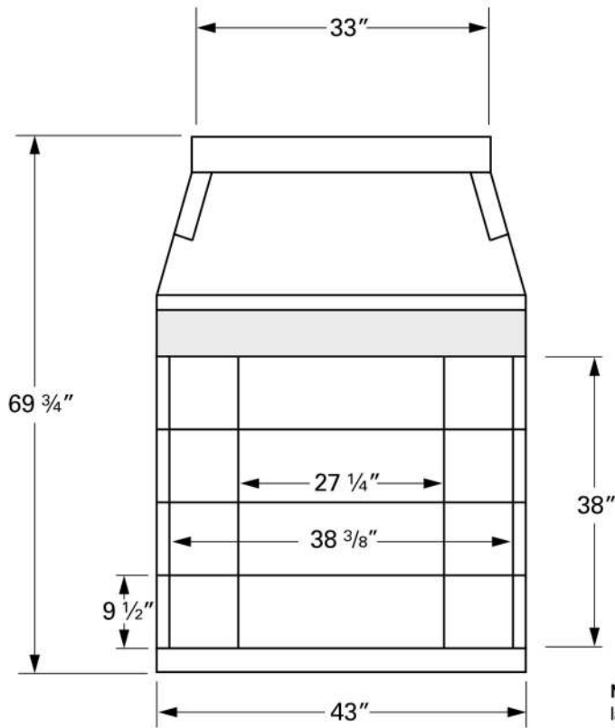
Vista frontal
