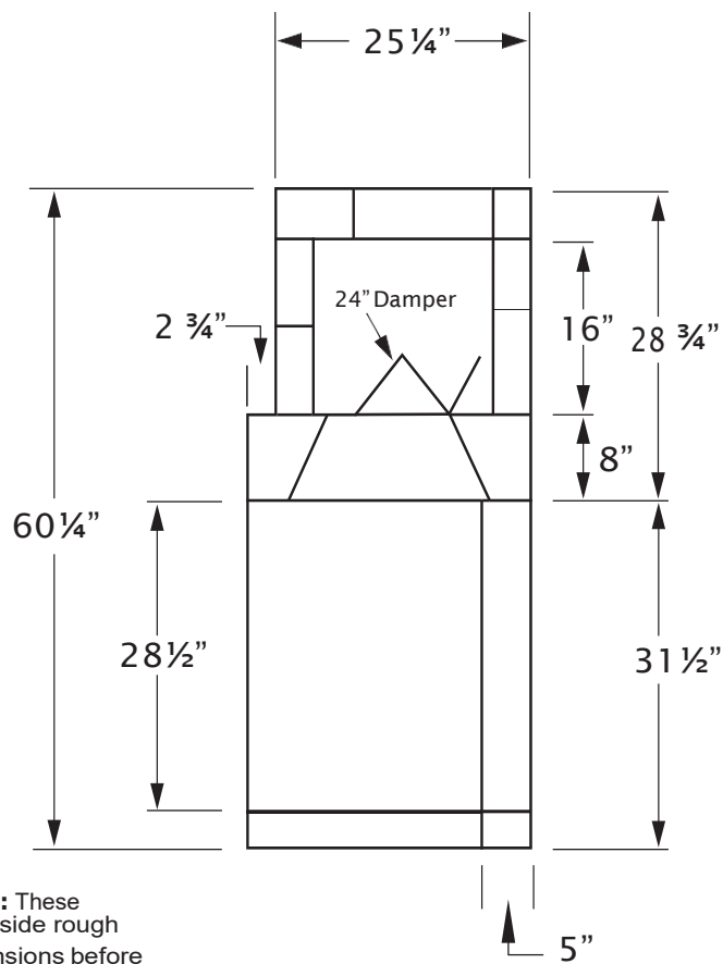
Side View
